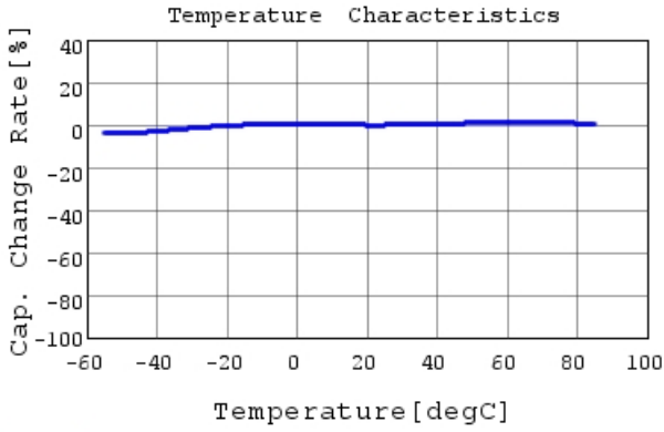
GRM155R61C224KA12 C-Temp. capchange, DC0.0V,
