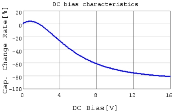
GRM155R61C224KA12 C-DC bias capchange, 25.0c
