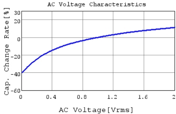
GRM155R61C224KA12 C-AC Voltage capchange, DC
