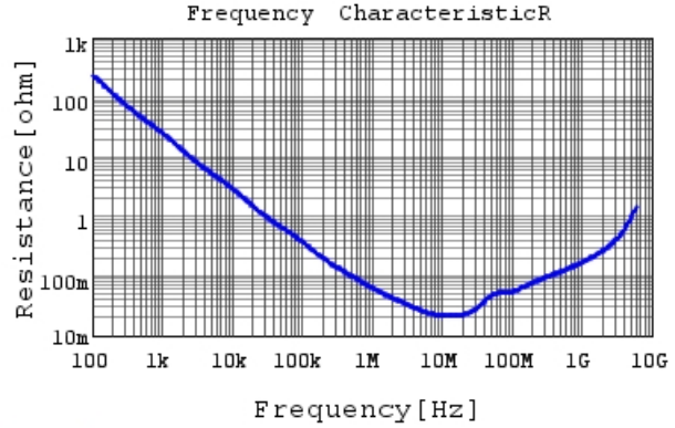
GRM155R61C224KA12 R DC0V, 25degC
