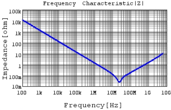
GRM155R61C224KA12 |Z| DC0V, 25degC
