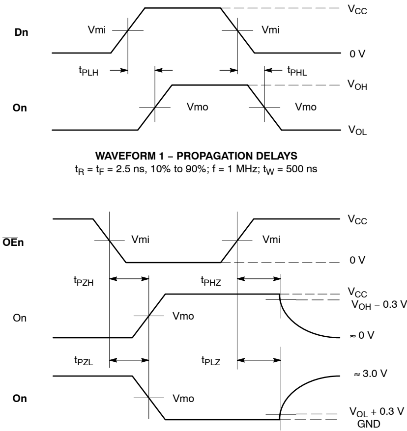
Figure 3. AC Waveforms
