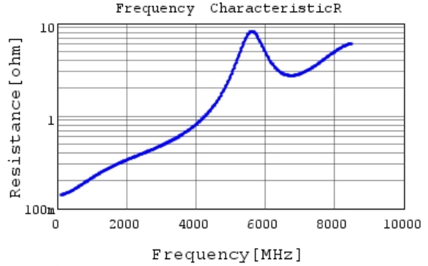
GRM1555C1H100JA01 R DCOV, 25degC
