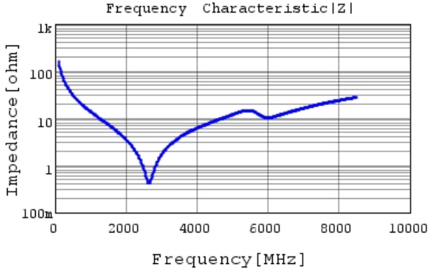
GRM1555C1H100JA01 |Z| DCOV, 25degC
