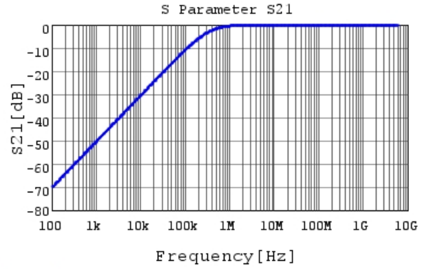
GCM188R71H472KA37 S21 DC0V, 25degC
