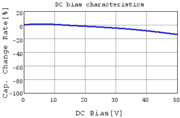
GCM188R71H472KA37 C-DC bias capchange, 25.0c
