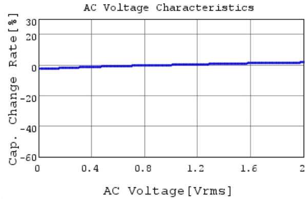
GCM188R71H472KA37 C-AC Voltage capchange, DC
