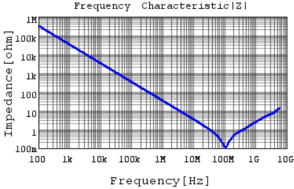
GCM188R71H472KA37 |Z| DC0V, 25degC
