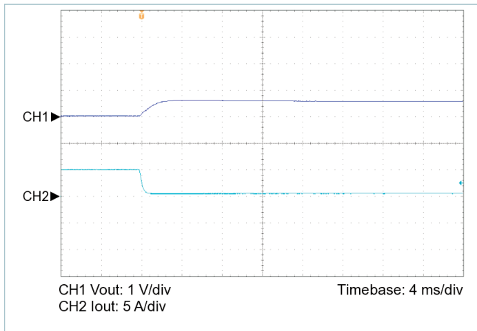
Figure 19 — 100% to 10% load transient response, V_{IN} = 30\text{ V} , nominal trim, C_{OUT\_EXT} = 1000\text{ }\mu\text{F}
