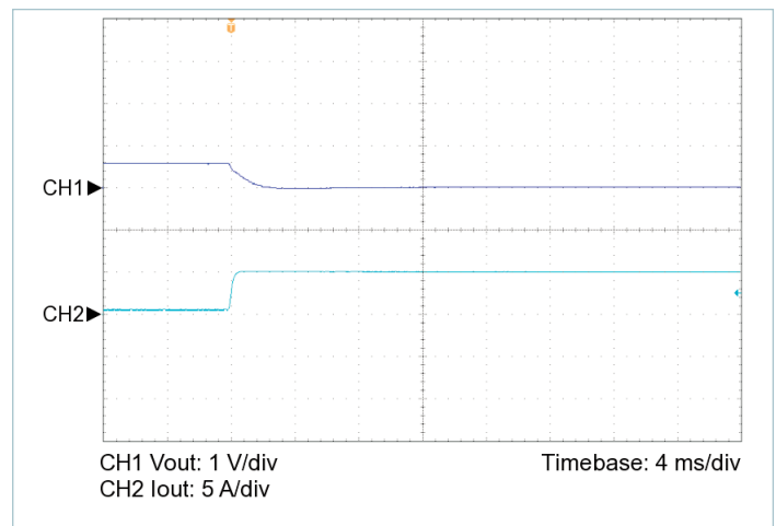
Figure 20 — 10% to 100% load transient response, V_{IN} = 30\text{ V} , nominal trim, C_{OUT\_EXT} = 1000\text{ }\mu\text{F}
