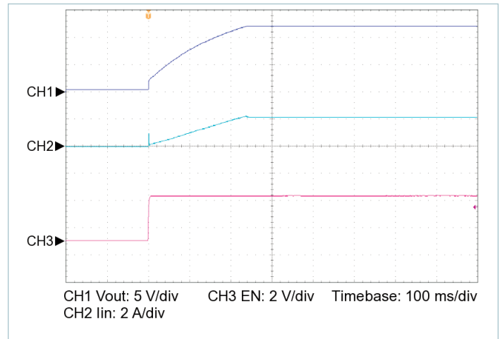
Figure 16 — Startup from EN, V_{IN} = 30\text{ V} , C_{OUT\_EXT} = 10000\text{ }\mu\text{F} , R_{LOAD} = 2.400\text{ }\Omega
