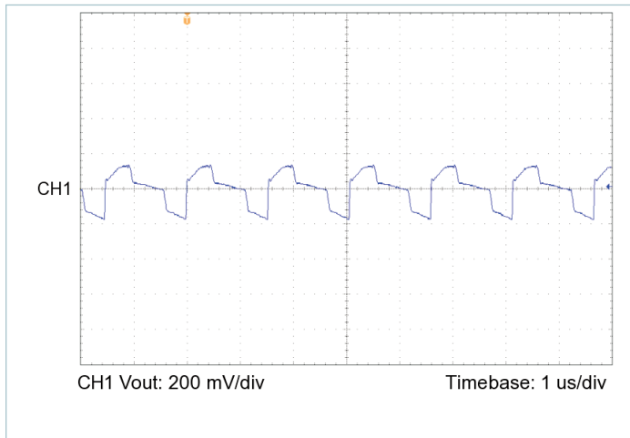
Figure 15 — Output voltage ripple, V_{IN} = 30\text{ V} , V_{OUT} = 12.0\text{ V} , C_{OUT\_EXT} = 1000\text{ }\mu\text{F} , R_{LOAD} = 2.400\text{ }\Omega
