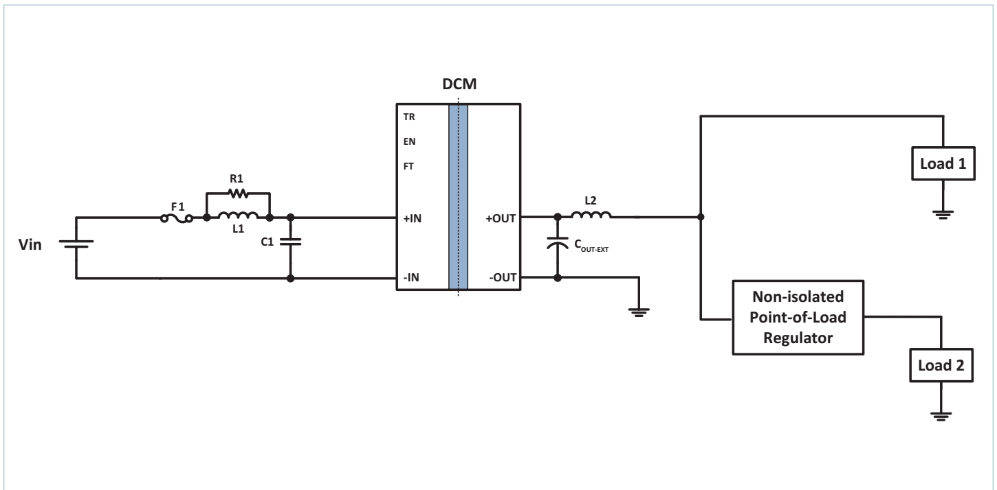
Typical Application: Single DCM3623x50M13C2y7z, to a non-isolated regulator, and direct to load
