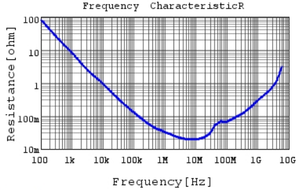
GCM188R71C104KA37 R DC0V, 25degC
