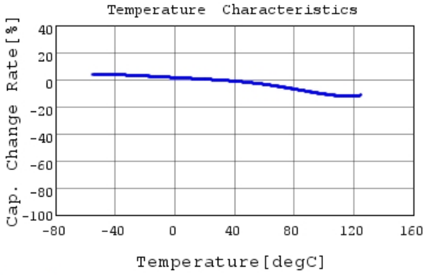
GCM188R71C104KA37 C-Temp. capchange, DC0.0V,
