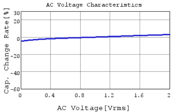
GCM188R71C104KA37 C-AC Voltage capchange, DC
