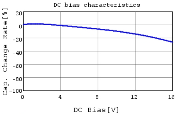
GCM188R71C104KA37 C-DC bias capchange, 25.0c
