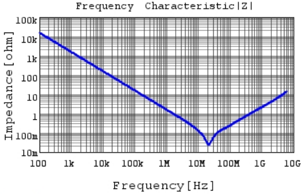
GCM188R71C104KA37 |Z| DC0V, 25degC
