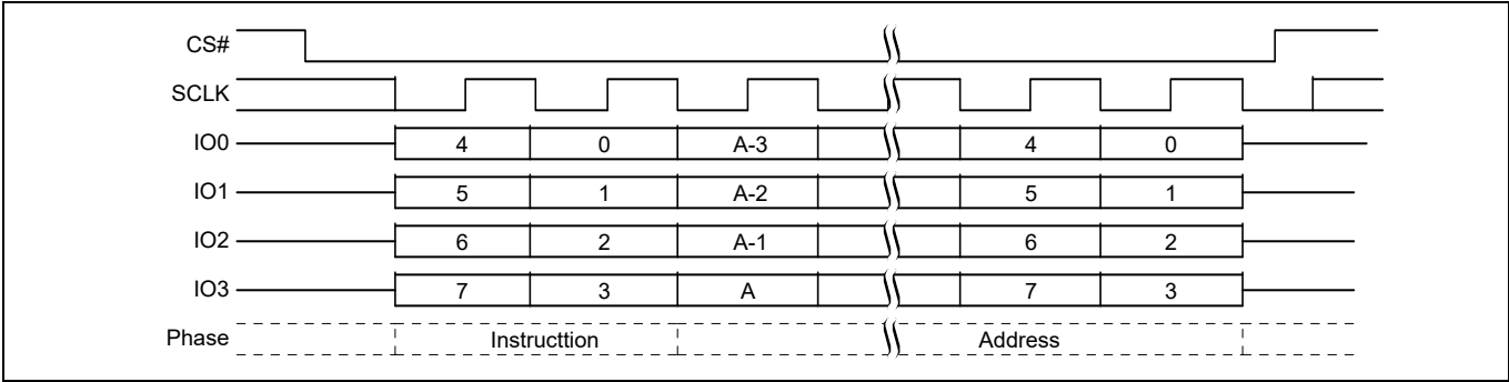
Figure 100 IBUL command sequence QPI mode [52, 53]
