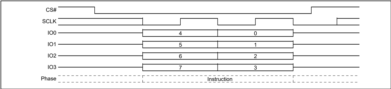
Figure 46 Write Enable for Volatile Registers (WREN) command sequence QPI mode
