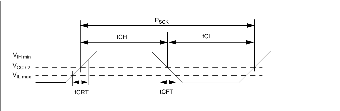
Figure 142 Clock timing
