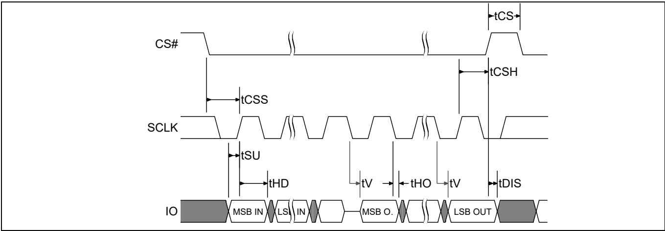
Figure 145 SDR MIO timing
