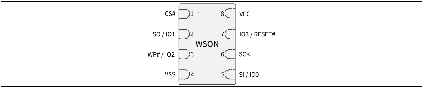
Figure 4 8-connector package (WSO5 5 x 6), top view [2]
