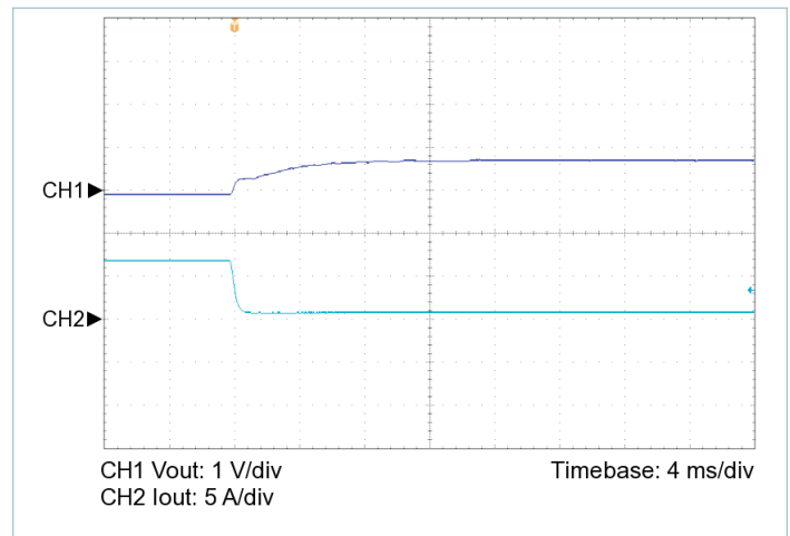
Figure 7 — 100% to 10% load transient response, V_{IN} = 30\text{ V} , nominal trim, C_{OUT\_EXT} = 470\text{ }\mu\text{F}
