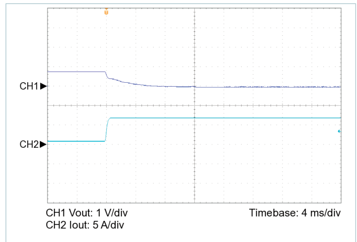
Figure 8 — 10% to 100% load transient response, V_{IN} = 30\text{ V} , nominal trim, C_{OUT\_EXT} = 470\text{ }\mu\text{F}
