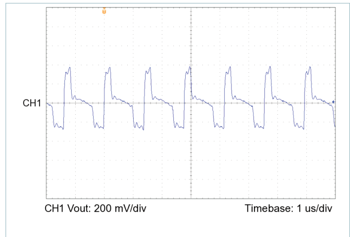
Figure 19 — Output voltage ripple, V_{IN} = 30\text{ V} , V_{OUT} = 24.0\text{ V} , C_{OUT\_EXT} = 470\text{ μF} , R_{LOAD} = 3.582\text{ Ω}
