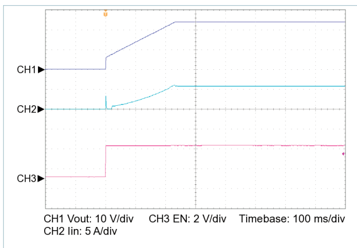
Figure 17 — Startup from EN, V_{IN} = 30\text{ V} , C_{OUT\_EXT} = 4700\text{ μF} , R_{LOAD} = 3.582\text{ Ω}
