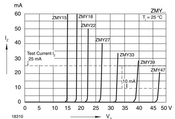
Fig. 6 - Breakdown Characteristics
