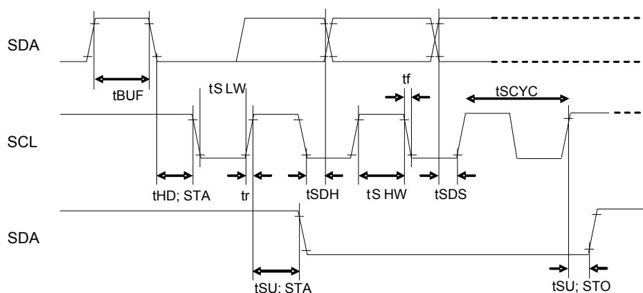
Figure 5. Interface Timing
