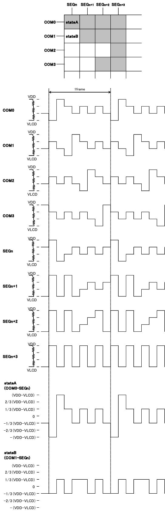
Figure 15. LCD Waveform at Line Inversion (1/3bias)
