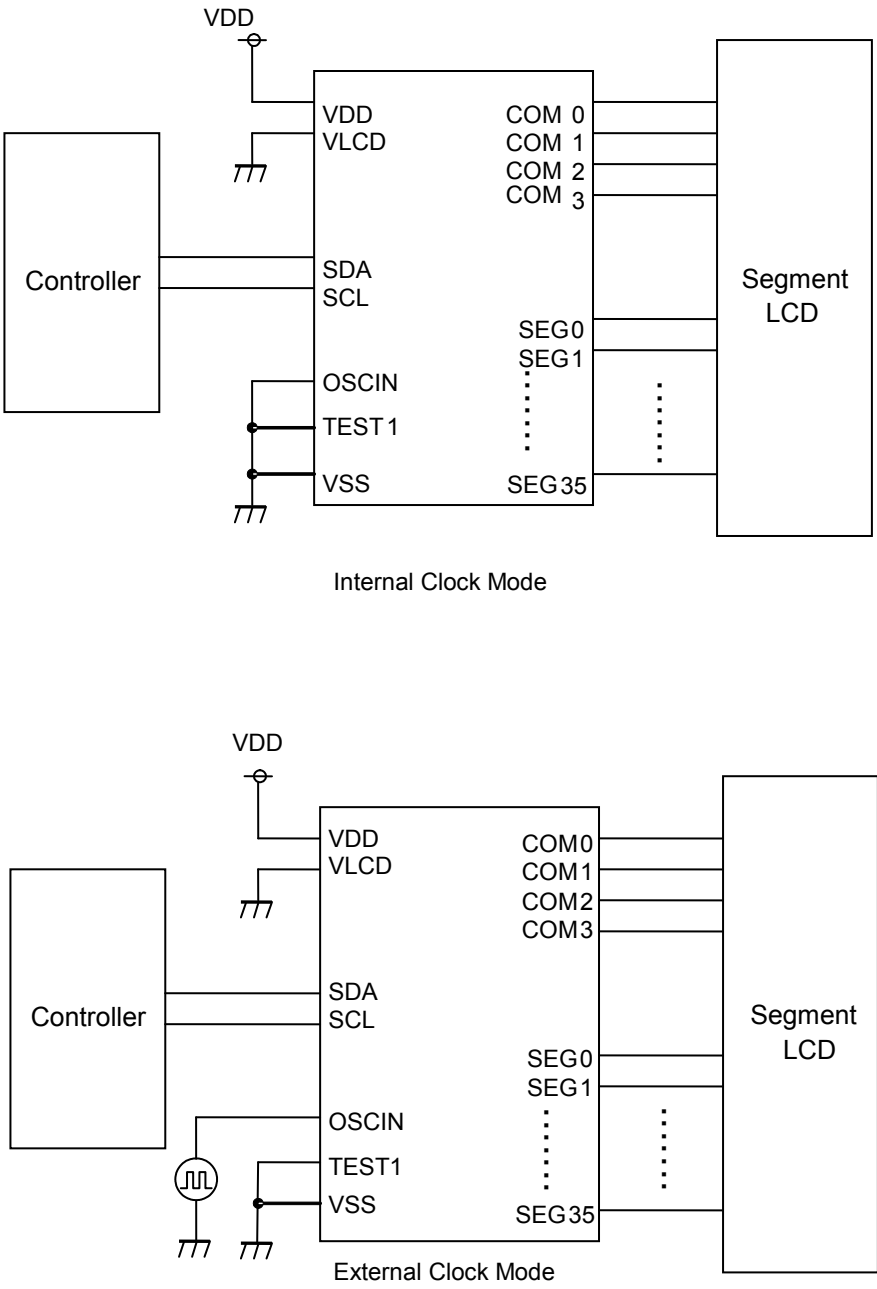
Figure 7. Example of Application Circuit
