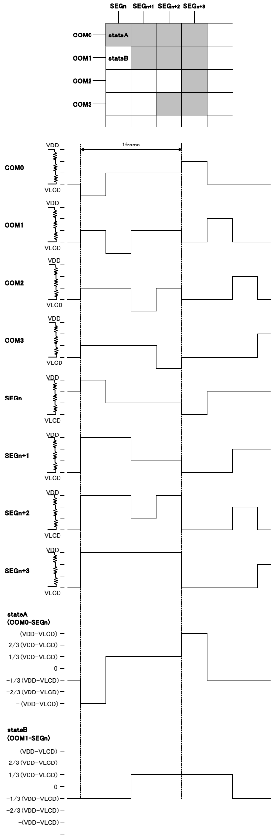
Figure 16. LCD Waveform at Frame Inversion (1/3bias)
