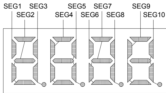
Figure 18. Example SEG Line Pattern
