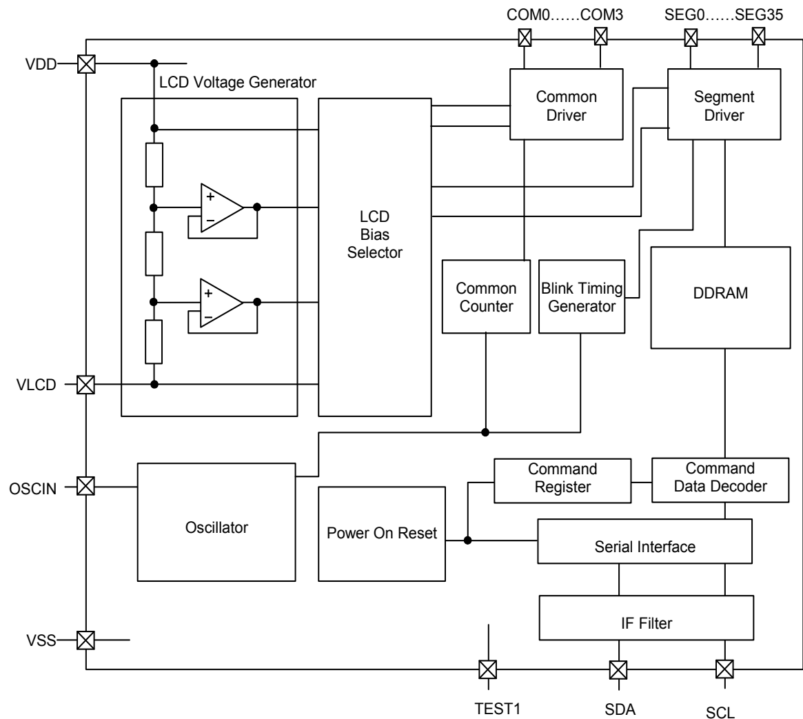
Figure 2. Block Diagram
