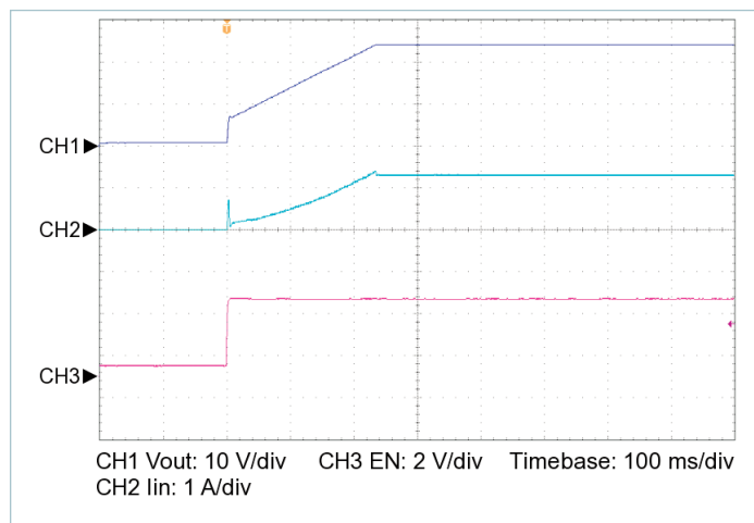
Figure 16 — Startup from EN, V_{IN} = 100\text{ V} , C_{OUT\_EXT} = 5000\text{ }\mu\text{F} , R_{LOAD} = 4.800\text{ }\Omega
