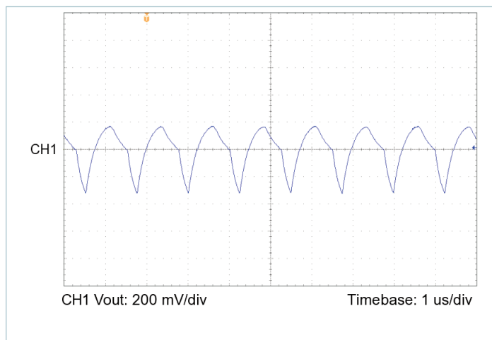
Figure 15 — Output voltage ripple, V_{IN} = 100\text{ V} , V_{OUT} = 24.0\text{ V} , C_{OUT\_EXT} = 470\text{ }\mu\text{F} , R_{LOAD} = 4.800\text{ }\Omega
