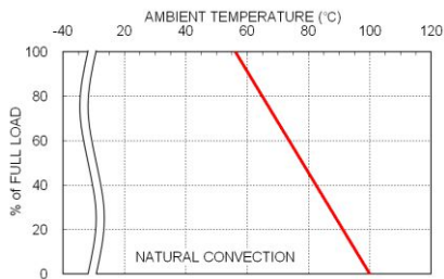
FDC20-48S05 Derating Curve
