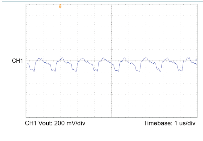
Figure 15 — Output voltage ripple, V_{IN} = 43\text{ V} , V_{OUT} = 28.0\text{ V} , C_{OUT\_EXT} = 470\text{ }\mu\text{F} , R_{LOAD} = 7.778\text{ }\Omega
