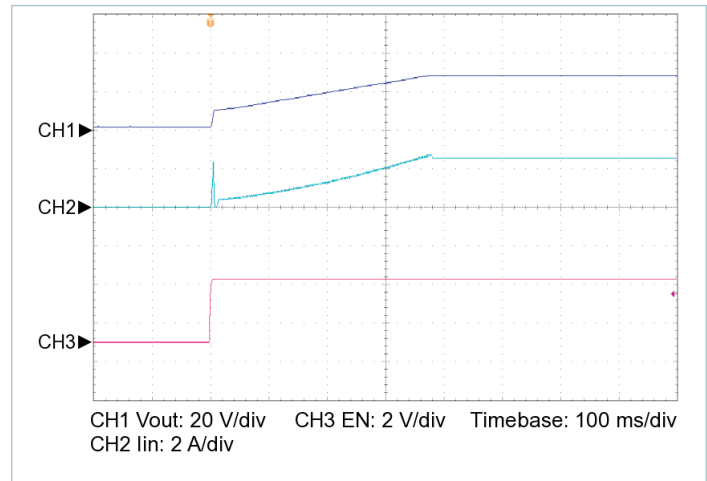
Figure 16 — Startup from EN, V_{IN} = 43\text{ V} , C_{OUT\_EXT} = 5000\text{ }\mu\text{F} , R_{LOAD} = 7.778\text{ }\Omega
