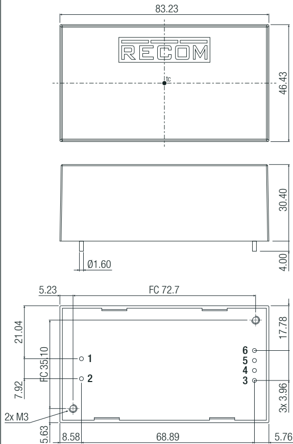
Dimension Drawing (mm)
