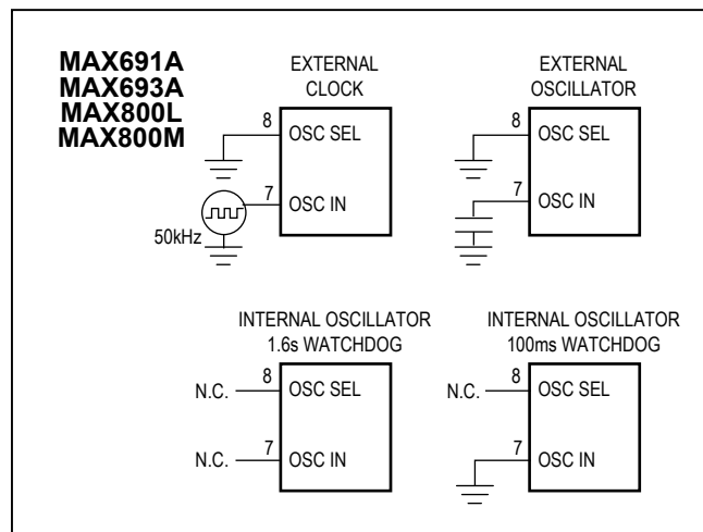
Figure 3. Oscillator Circuits
