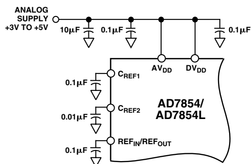
Figure 16. Relevant Connections Using Internal Reference
