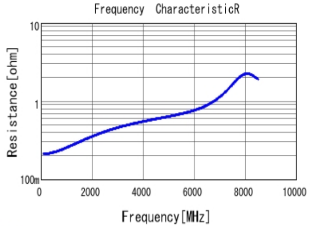
■ GRM1555C1H4R7CA01 R DC0V, 25degC
