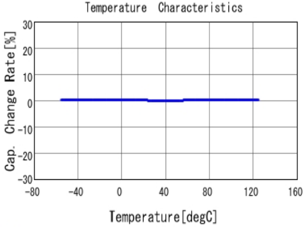
■ GRM1555C1H4R7CA01 C-Temp. capchange, DCOV, AC1Vrms
