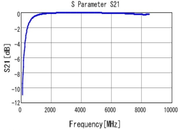
■ GRM1555C1H4R7CA01 S21 DCOV, 25degC
