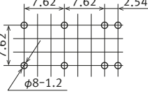
Recommended PC board pattern (BOTTOM VIEW)
