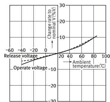
4-3. Ambient temperature characteristics (2 Form A: Average)
