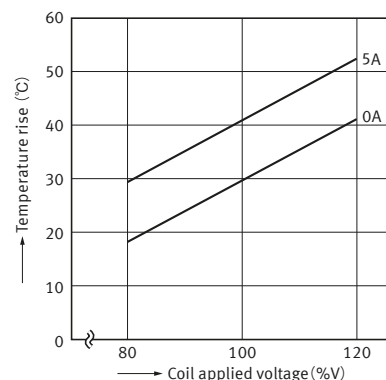
3-3. Coil temperature characteristics (2 Form A: Average)
