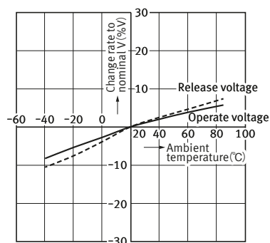
4-1. Ambient temperature characteristics (1 Form A: Average)
