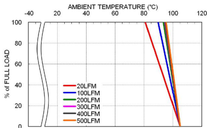
LCD10-48S05 Derating Curve
