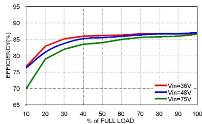
LCD10-48S05 Efficiency vs. Output Load
