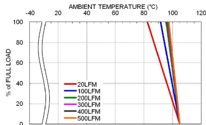
LCD10-48S05 Derating Curve With Heat-sink
