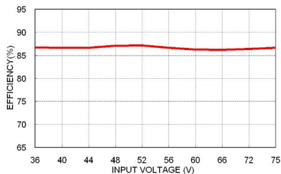
LCD10-48S05 Efficiency vs. Input Voltage
