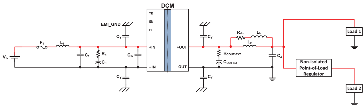
Typical Application 2: Single DCM4623xD2K53E0yzz, to a non-isolated regulator, and direct to load
