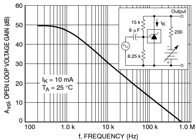
Figure 15. Open-Loop Voltage Gain versus Frequency
