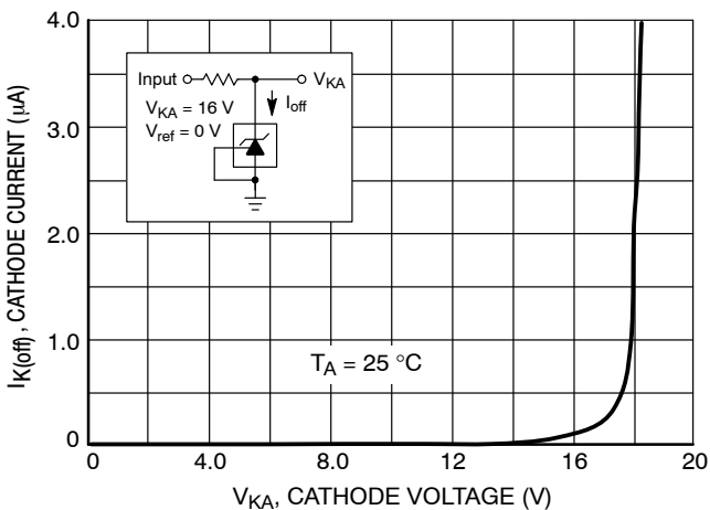
Figure 11. Off-State Cathode Current versus Cathode Voltage
