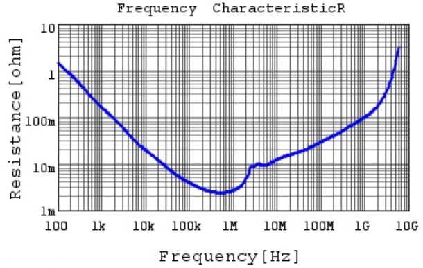
GRM21BR61A226ME44 R DCOV, 25degC
