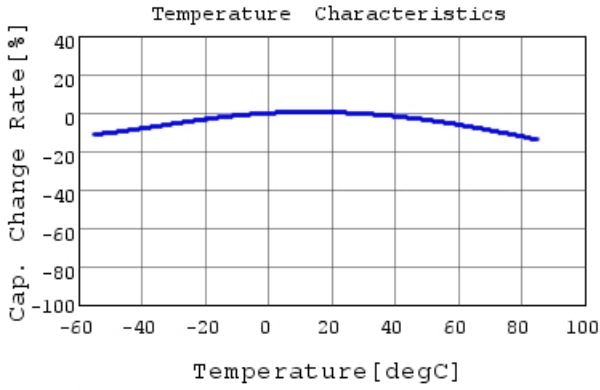
GRM21BR61A226ME44 C-Temp. capchange, DC0.0V,
