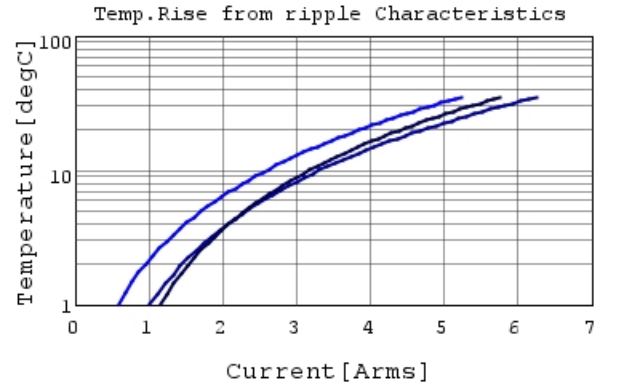
GRM21BR61A226ME44 Temp.rise — 80kHz
