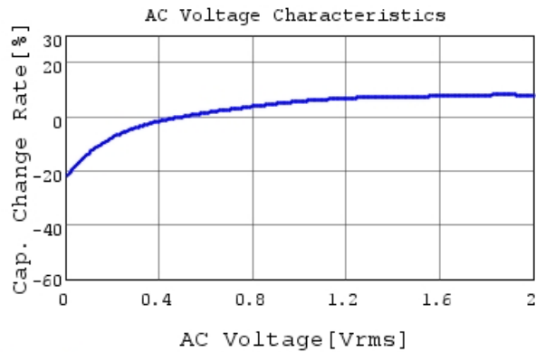
GRM21BR61A226ME44 C-AC Voltage capchange, DC
