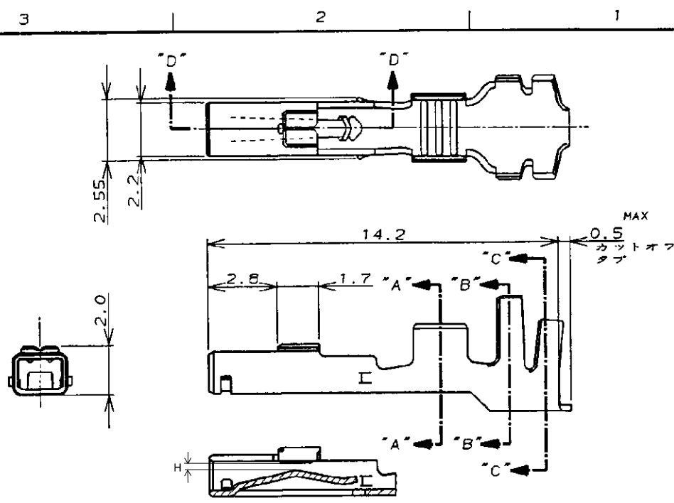
断面 "D"- "D" SECT
