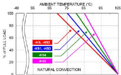
QAE40-72S05U Derating Curve with Heat-sink (See Thermal Considerations)
