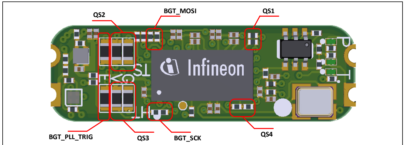
Figure 15 MMIC QS1 to QS4 quad state inputs
