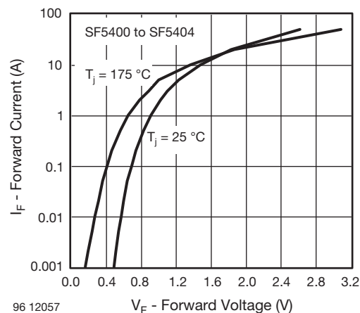
Fig. 6 - Max. Forward Current vs. Forward Voltage
