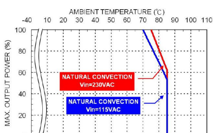
Derating Curve vs. Ambient Temperature MAD30USxxB xx=12/15/24/28/36/48/53 Connector Option : (□: JST)
