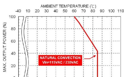
Derating Curve vs. Ambient Temperature MAD30USxxB xx=3P3/05/7P5/09/121/151/18 Connector Option : (□: JST)
