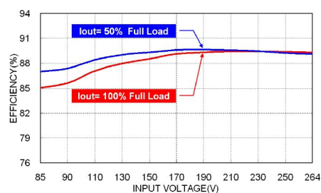
MAD30US24B Efficiency vs. Input Voltage
