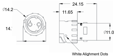
Plug Connector, Free-Hanging
