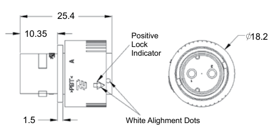
Cap Connector, Free-Hanging
