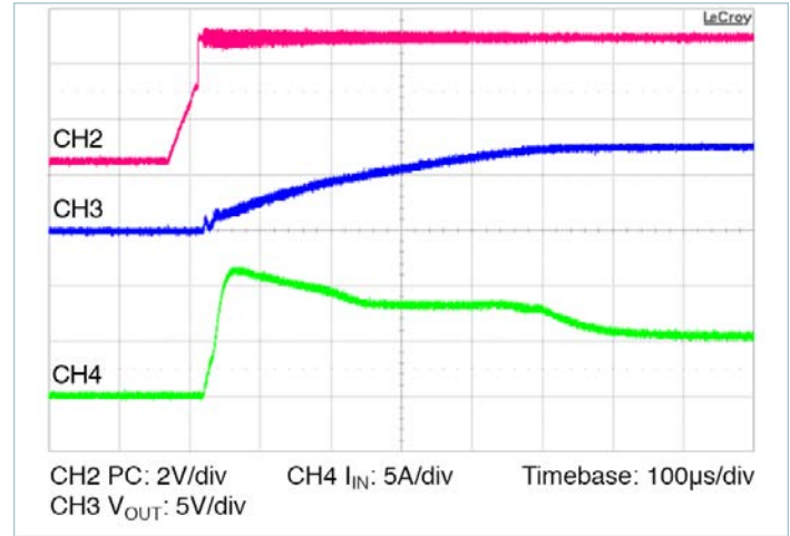
Figure 13 — Start up from application of PC; V_{IN} pre-applied C_{OUT} = 2300\mu\text{F}
