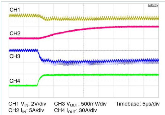
Figure 14 — 0 – 30A transient response: C_{IN} = 330\mu\text{F} , I_{IN} measured prior to C_{IN} , no external C_{OUT}
