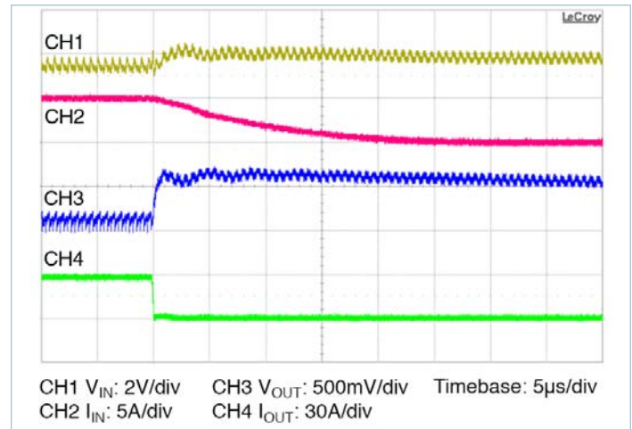
Figure 15 — 30 – 0A transient response: C_{IN} = 330\mu\text{F} , I_{IN} measured prior to C_{IN} , no external C_{OUT}
