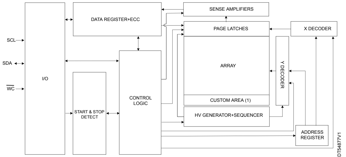
Figure 4. Block diagram
