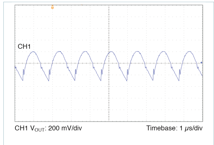
Figure 19 — Output voltage ripple, V_{IN} = 270\text{ V} , V_{OUT} = 12.0\text{ V} , C_{OUT\_EXT} = 1000\text{ }\mu\text{F} , R_{LOAD} = 0.288\text{ }\Omega
