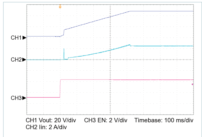
Figure 16 — Startup from EN, V_{IN} = 43\text{ V} , C_{OUT\_EXT} = 2200\text{ }\mu\text{F} , R_{LOAD} = 22.857\text{ }\Omega
