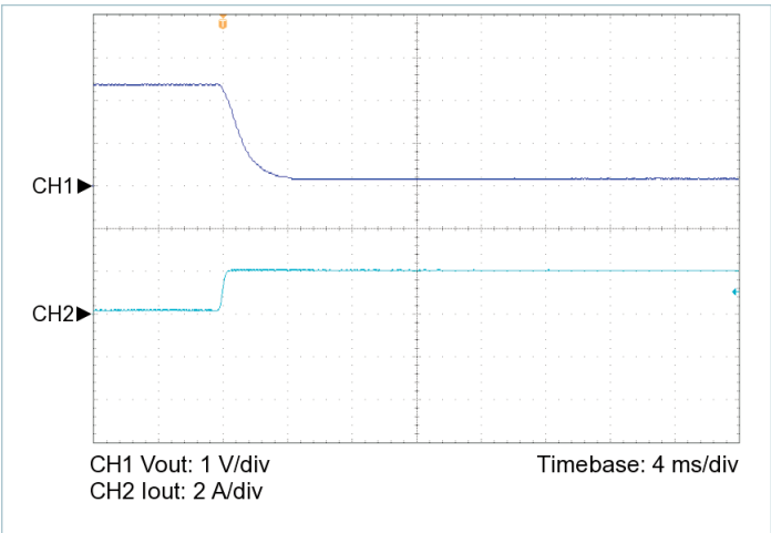
Figure 20 — 10% to 100% load transient response, V_{IN} = 43\text{ V} , nominal trim, C_{OUT\_EXT} = 220\text{ }\mu\text{F}
