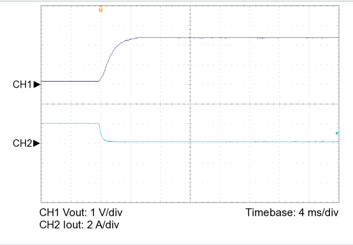
Figure 19 — 100% to 10% load transient response, V_{IN} = 43\text{ V} , nominal trim, C_{OUT\_EXT} = 220\text{ }\mu\text{F}
