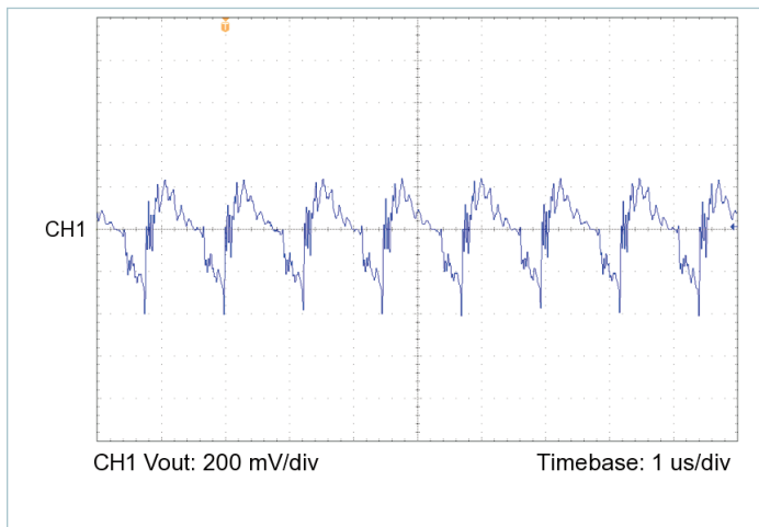
Figure 15 — Output voltage ripple, V_{IN} = 43\text{ V} , V_{OUT} = 48.0\text{ V} , C_{OUT\_EXT} = 220\text{ }\mu\text{F} , R_{LOAD} = 22.857\text{ }\Omega
