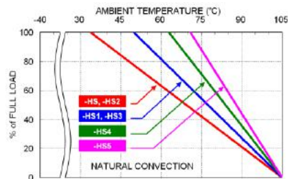
QAE100-48S05 Derating Curve with Heat-sink (See Thermal Considerations)
