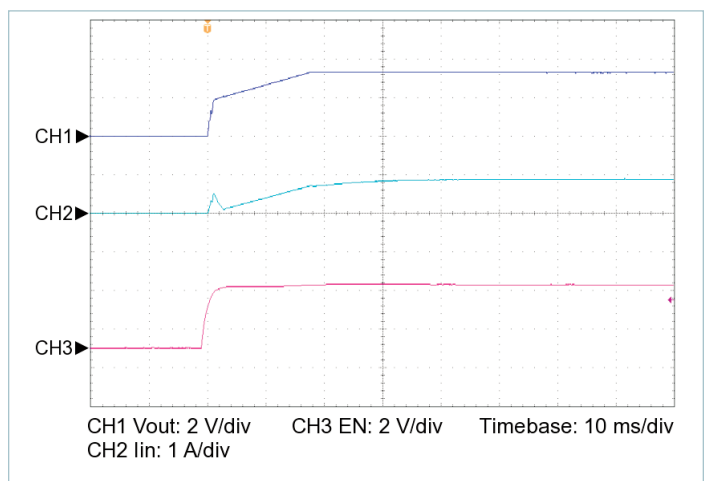
Figure 14 — Startup from EN, V_{IN} = 100\text{ V} , C_{OUT\_EXT} = 20000\text{ }\mu\text{F} , R_{LOAD} = 0.136\text{ }\Omega
