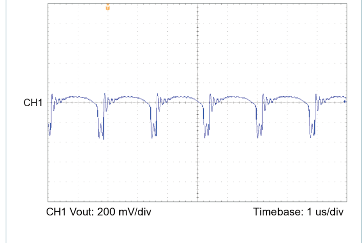
Figure 16 — Output voltage ripple, V_{IN} = 100\text{ V} , V_{OUT} = 3.3\text{ V} , C_{OUT\_EXT} = 1000\text{ }\mu\text{F} , R_{LOAD} = 0.136\text{ }\Omega
