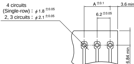
Inner-housing lock
