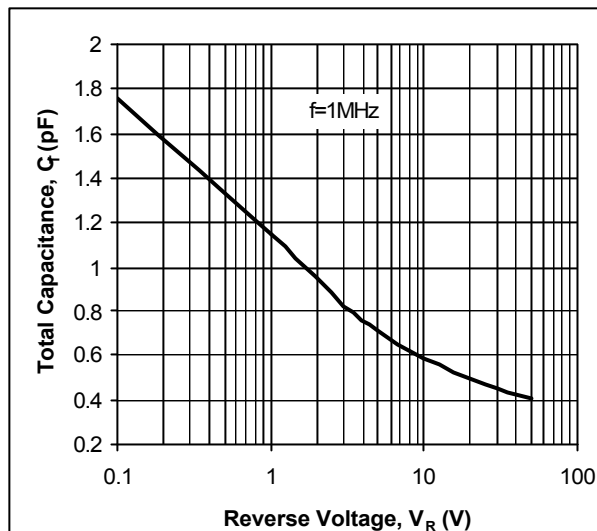
Fig. 3. Typical Capacitance
