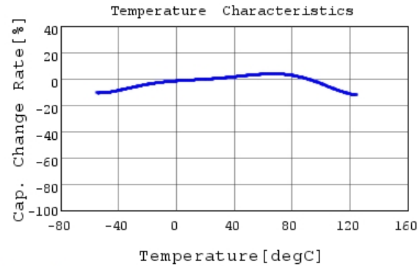
GRM21BR71A475KE51 C-Temp. capchange, DC0.0V,
