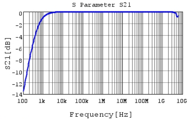
GRM21BR71A475KE51 S21 DC0V, 25degC
