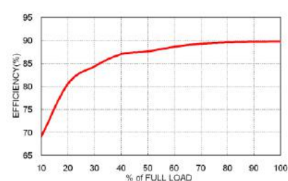
UFED40-48S05W Efficiency vs. Output Load
