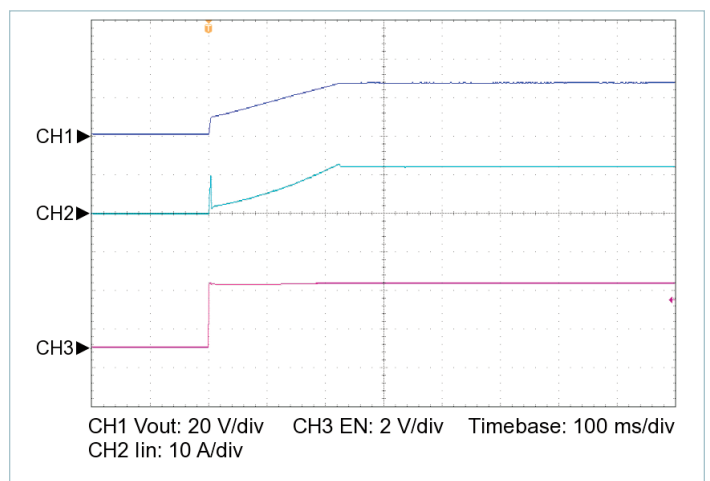
Figure 14 — Startup from EN, V_{IN} = 28\text{ V} , C_{OUT\_EXT} = 10000\text{ }\mu\text{F} , R_{LOAD} = 2.450\text{ }\Omega
