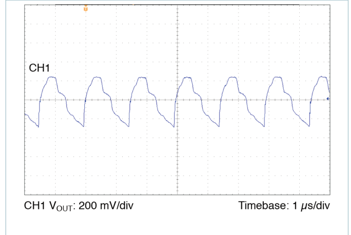
Figure 16 — Output voltage ripple, V_{IN} = 28\text{ V} , V_{OUT} = 28.0\text{ V} , C_{OUT\_EXT} = 1000\text{ }\mu\text{F} , R_{LOAD} = 2.450\text{ }\Omega
