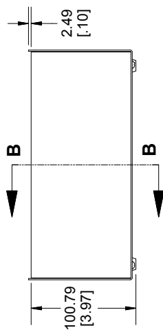
BACK VIEW OF ENCLOSURE
