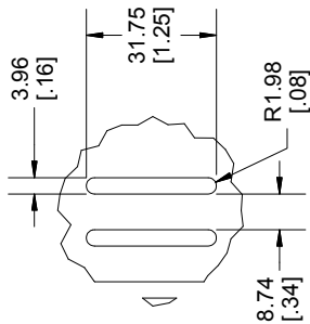
DETAIL A SCALE 1 / 2 END VENTS
