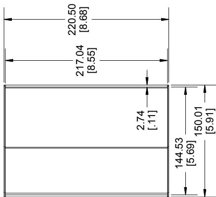
TOP VIEW OF ENCLOSURE
