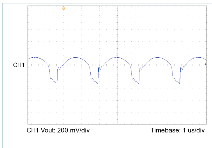
Figure 19 — Output voltage ripple, V_{IN} = 28\text{ V} , V_{OUT} = 3.3\text{ V} , C_{OUT\_EXT} = 1000\text{ μF} , R_{LOAD} = 0.091\text{ Ω}
