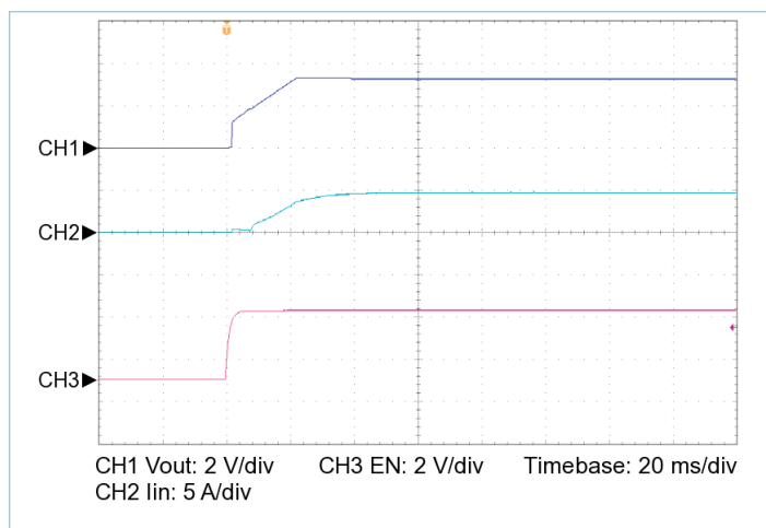
Figure 17 — Startup from EN, V_{IN} = 28\text{ V} , C_{OUT\_EXT} = 20000\text{ μF} , R_{LOAD} = 0.091\text{ Ω}
