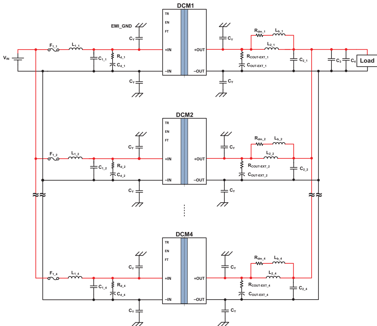
Typical Application 1: DCM3623x50M04A2yzz in an array of four units
