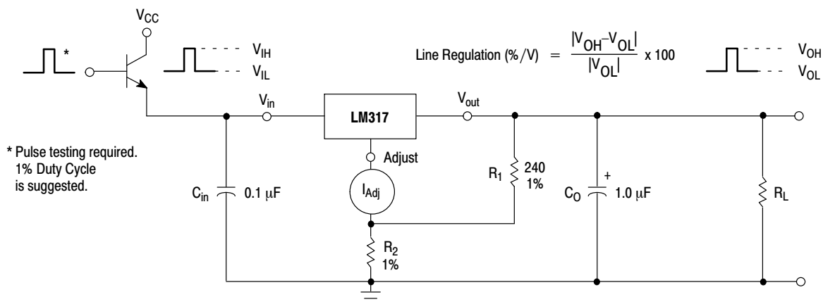
Figure 3. Line Regulation and \Delta I_{Adj}/Line Test Circuit
