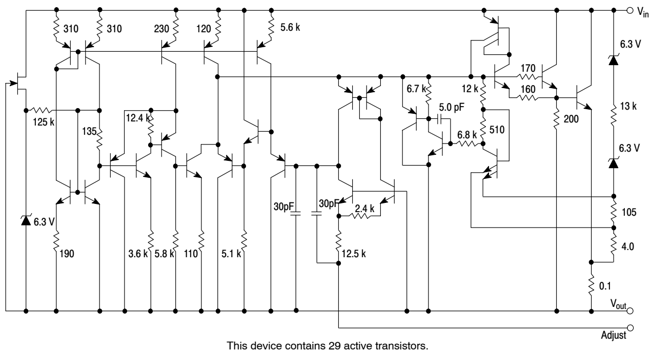
Figure 2. Representative Schematic Diagram
