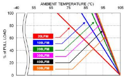
RED40-24S05W Derating Curve
