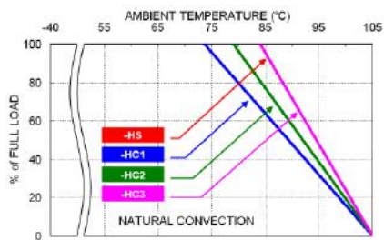
RED40-24S05W Derating Curve With Heat-sink
