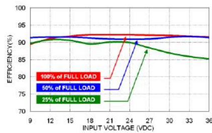
RED40-24S05W Efficiency vs. Input Voltage
