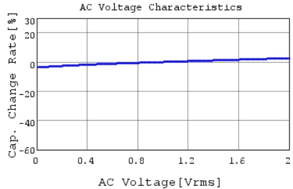
GRT21BR71H105KE01 C-AC Voltage capchange, Dc
