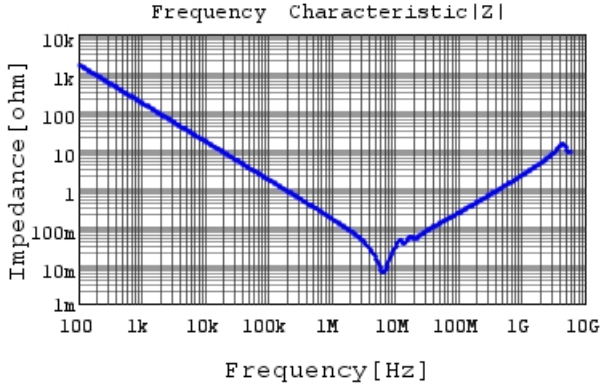
GRT21BR71H105KE01 |Z| DCOV, 25degC
