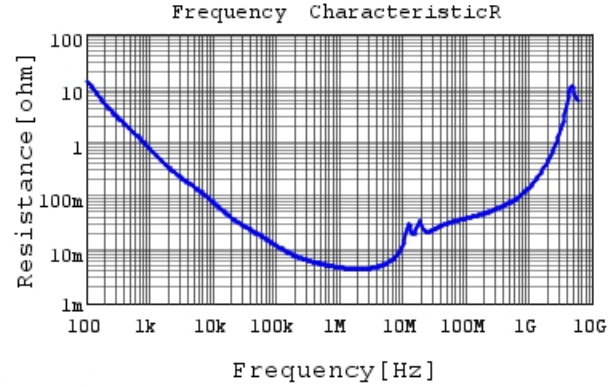
GRT21BR71H105KE01 R DCOV, 25degC
