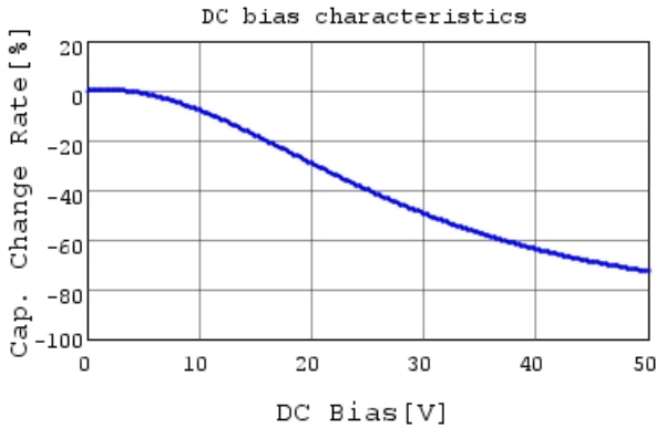
GRT21BR71H105KE01 C-DC bias capchange, 25.0c
