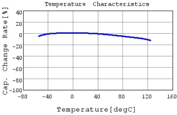
GRT21BR71H105KE01 C-Temp. capchange, DC0.0V,
