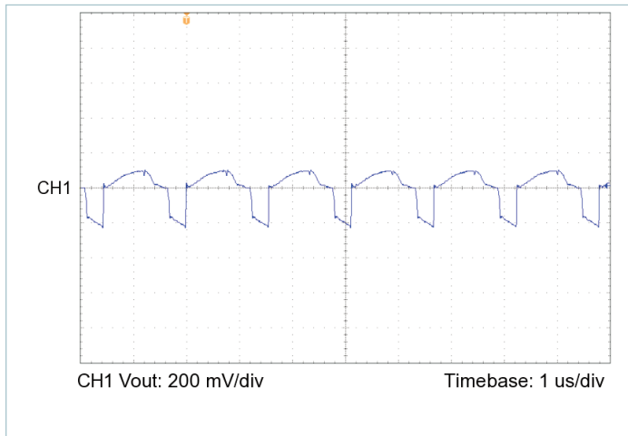
Figure 15 — Output voltage ripple, V_{IN} = 43\text{ V} , V_{OUT} = 5.0\text{ V} , C_{OUT\_EXT} = 1000\text{ }\mu\text{F} , R_{LOAD} = 0.500\text{ }\Omega
