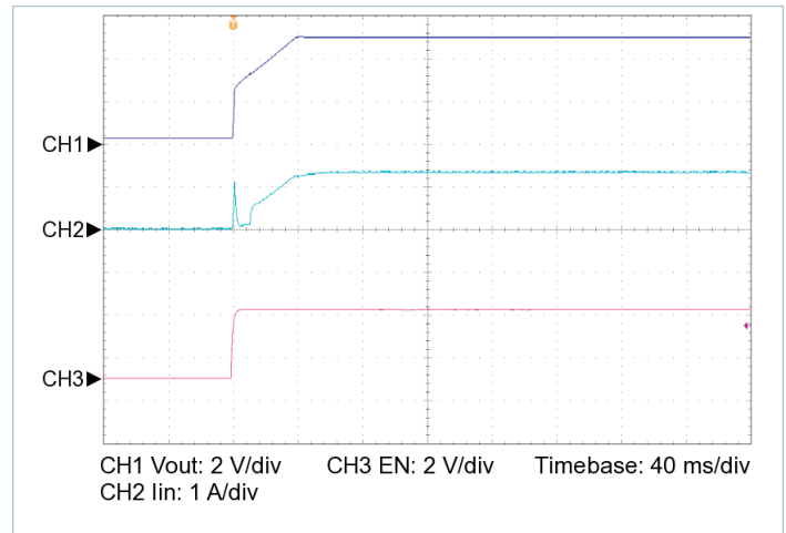
Figure 16 — Startup from EN, V_{IN} = 43\text{ V} , C_{OUT\_EXT} = 10000\text{ }\mu\text{F} , R_{LOAD} = 0.500\text{ }\Omega
