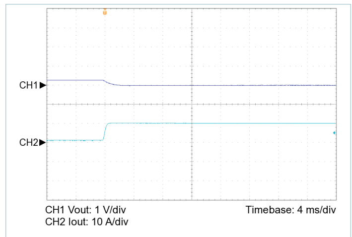
Figure 20 — 10% to 100% load transient response, V_{IN} = 43\text{ V} , nominal trim, C_{OUT\_EXT} = 1000\text{ }\mu\text{F}
