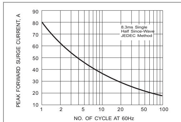
Fig.10 Maximum Non-Repetitive Surge Current
