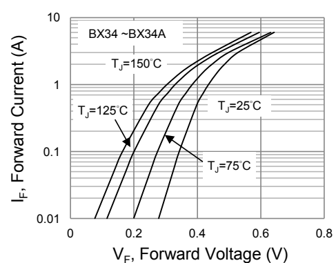
Fig.6 Typical Forward Characteristics
