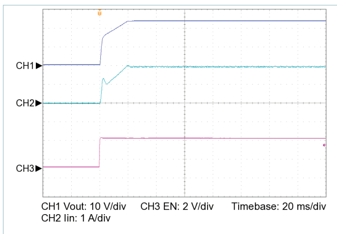
Figure 17 — Startup from EN, V_{IN} = 270\text{ V} , C_{OUT\_EXT} = 2200\text{ }\mu\text{F} , R_{LOAD} = 1.152\text{ }\Omega
