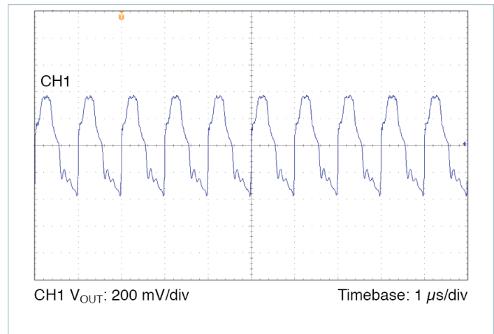
Figure 19 — Output voltage ripple, V_{IN} = 270\text{ V} , V_{OUT} = 24.0\text{ V} , C_{OUT\_EXT} = 220\text{ }\mu\text{F} , R_{LOAD} = 1.152\text{ }\Omega
